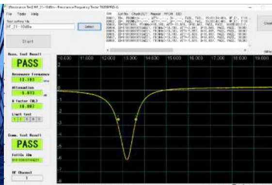
Freq/Q-Factor
